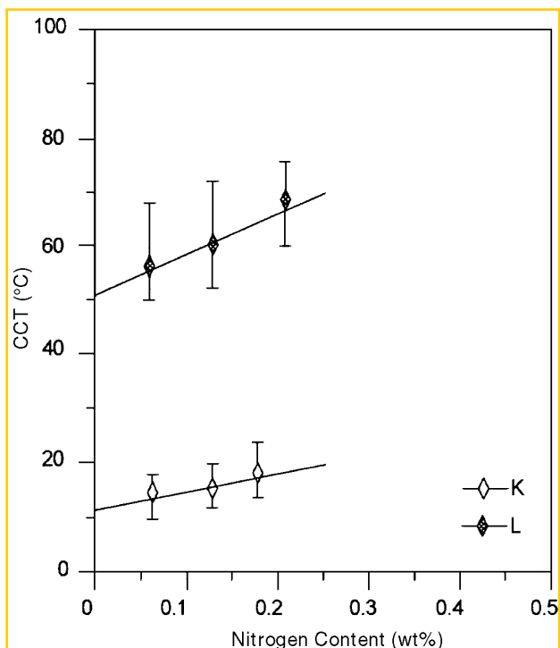
FIGURE 5. CCT in 0.2 M NaCl at 600 mV_{SCE} for a clamped metal metal crevice, plotted as a function of nitrogen content. Error bars denote maximum and minimum measured values, and lines show values calculated using Equation (6)
